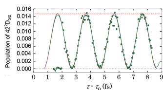
Figure 3. Time domain Ramsey interferometry of ultracold ^{87}\text{Rb} atoms with attosecond precision to be used as a readout interface of the ultrafast quantum simulator.
