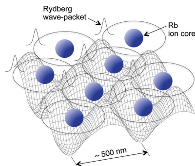
Figure 1. Metal-like quantum gas. A schematic of the many-body system of ultracold Rydberg atoms, where electronic wave functions spatially overlap between neighboring atoms. 2,7)
