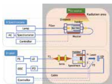
Figure 3. Experimental setup for spectroscopy (A: Spectroscopy), and laser properties measurement (B: Laser). Controller: temperature controller; ED: energy detector; H: Heater; Holder: specimen holder; OSC: oscilloscope; PD 1,2: photodiode; PS: power supply; and S: temperature sensor.
