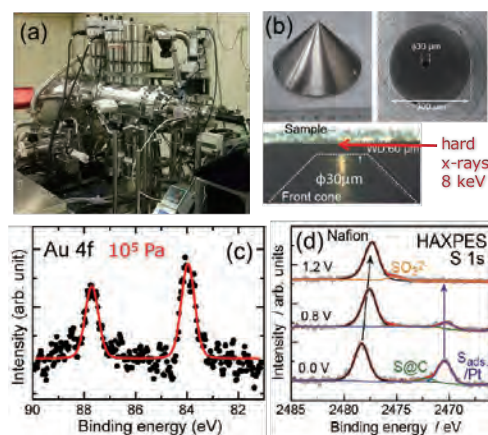
Ambient pressure hard x-ray photoelectron spectroscopic system. (a) Apparatus installed at SPring-8 Beamline 36XU. (b) Front cone with a 30- \mu m aperture of the electron energy analyzer, made by Equipment Development Center, IMS. (c) Au 4f HAXPES of Au(111) at a real ambient pressure of 10^5 Pa. (d) S 1s HAXPES of polymer electrolyte fuels cells under working conditions of the cathode-anode voltages of 0.0, 0.8 and 1.2 V.
