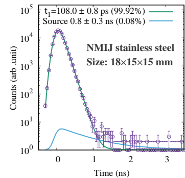
Fig.2: Positron annihilation lifetime spectrum of stainless steel for positron defect measurements (5607-a) supplied by National Metrology Institute of Japan (NMIJ). Measured positron lifetime 108 ps agrees well with the indicative value.
