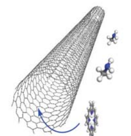
Functionalization by doping.
