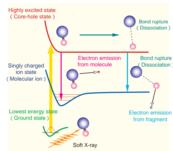
A schematic representation of molecular core excitation and its subsequent decay processes.
