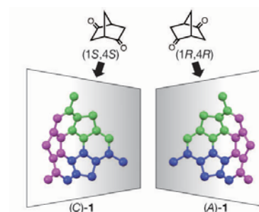
Synthesis of homochiral Buckybowls.
