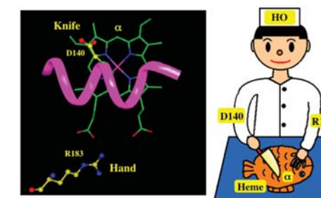
Molecular mechanism of heme oxygenase.
