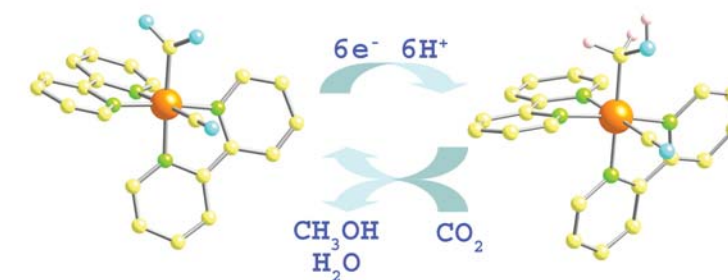
Multi-electron reduction of CO 2 .
