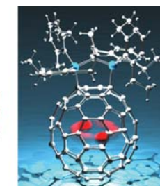
Control of rotational motion by chemical modification and application to molecular devices.
