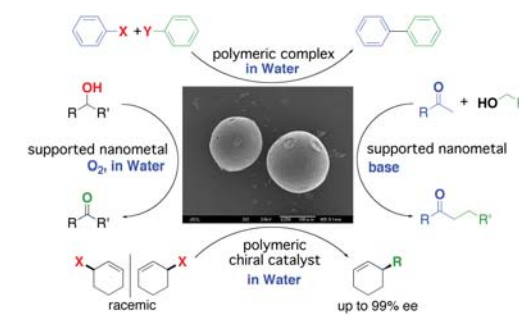
Typical Examples of Heterogeneous Aquacatalyses using Amphilic Polymer-Supported Metal Complexes and Metal Nanoparticles: A typical SEM image of the polymeric catalyst (center); C-C bond forming catalysis (top); aerobic alcohol oxidation (left); -alkylation with alcohol (right); asymmetric allylic substitution (bottom).
