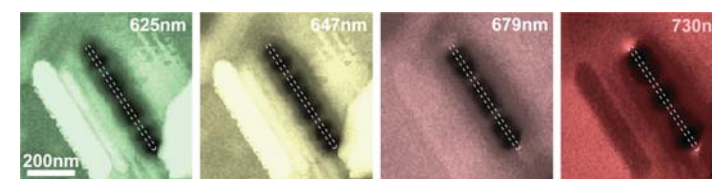
Near-field optical images of a nanometer-sized (length 510nm) metal rod. Wave function is visualized and is dependent on the wavelength observed.
