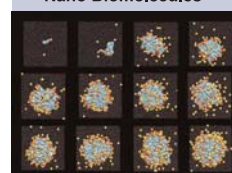
Drug Delivery System (Molecular Dynamics of Micelles)
