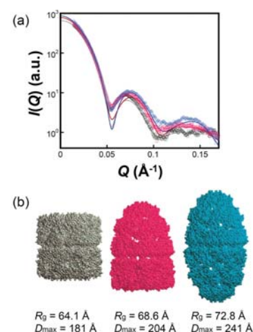
(a) Small-angle X-ray scattering patterns of molecular chaperones, GroEL and the GroEL-GroES complexes. (b) The three-dimensional structures of GroEL (gray), the bullet-type GroEL-GroES complex (magenta), and the football-type GroEL-GroES complex (cyan)(Inobe et al., Biophys. J. 94: 1392-1402 (2008)).
