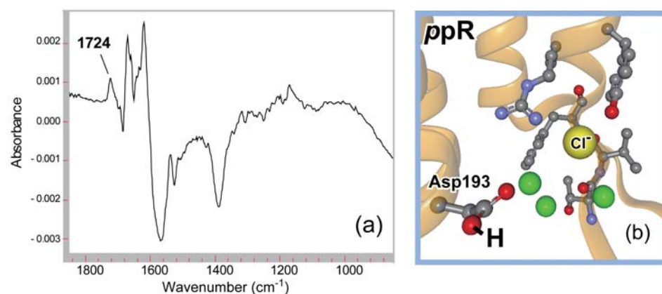
(a) Chloride-ion binding induced difference infrared spectra of a membrane protein ( pharaonis phoborhodopsin; light sensor in an archaeobacterium). The 1724-cm -1 band was assigned to the protonated carboxylate group of Asp193.
