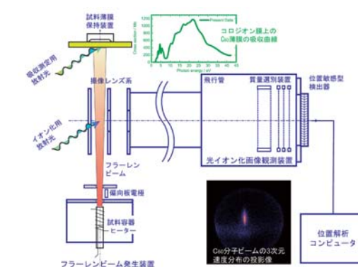
Apparatuses developed by our group for the velocity map imaging of C_{60} molecular beam and extreme UV photoabsorption of C_{60} thin film. In 2008 data from these machines were published for the first time.
