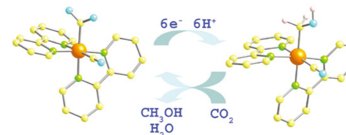
Multi-electron reduction of \text{CO}_2 .
