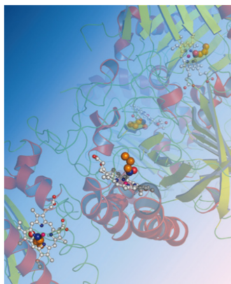
Structure of a novel heme enzyme, aldoxime dehydratase (OxdRE).
