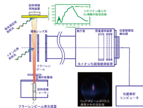
Apparatuses developed by our group for the velocity map imaging of C 60 molecular beam and extreme UV photoabsorption of C 60 thin film. In 2008 data from these machines were published for the first time.
