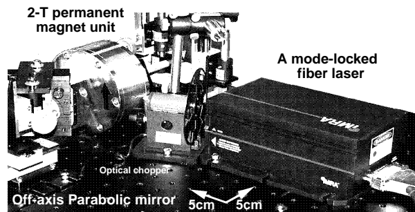
Figure 1. Photograph of a compact THz-radiation source with a bulk semiconductor, a fiber femtosecond laser, and a 2-T permanent magnet. Including the laser, the size is less than 40 × 30 × 15 cm.
