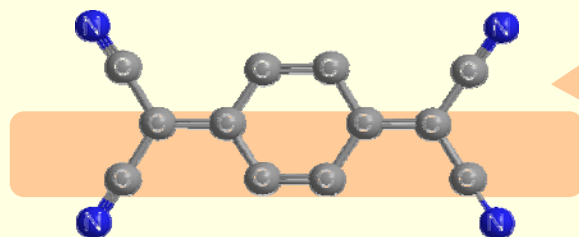
Tetracyanoquinodimethan (TCNQ)
